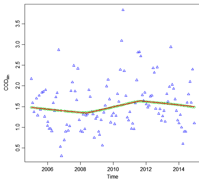
Fig. 5 LWPR-SegReg of monthly irregular and discrete \text{COD}_{\text{Mn}} concentrations. Blue triangles are original \text{COD}_{\text{Mn}} data, green circles are pretreated \text{COD}_{\text{Mn}} time series derived from LWPR, and red line is the SegReg results of the pretreated \text{COD}_{\text{Mn}} time series
